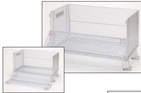
Left: Wire Mesh Folding Junior Container with 1/2" x 1/2" mesh. The large picture reflects the double-drop gate folded half way. The smaller picture reflects double-drop gate fully dropped.
