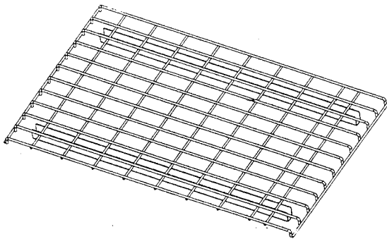
Wire mesh rack decking with a waterfall for step beam applications: 2" x 4" mesh
