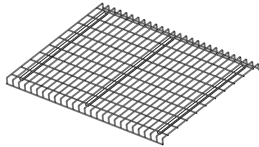
Wire Mesh Deck to Fit 5/8" Step, Standard Top Width of Beam
